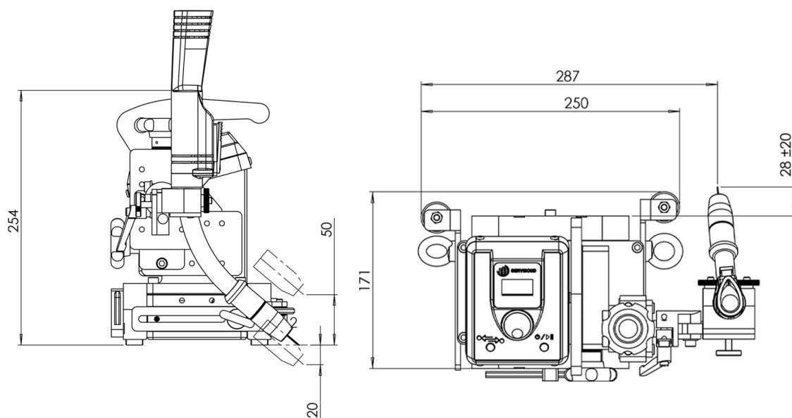
MAGLIGHT ORIGINAL
